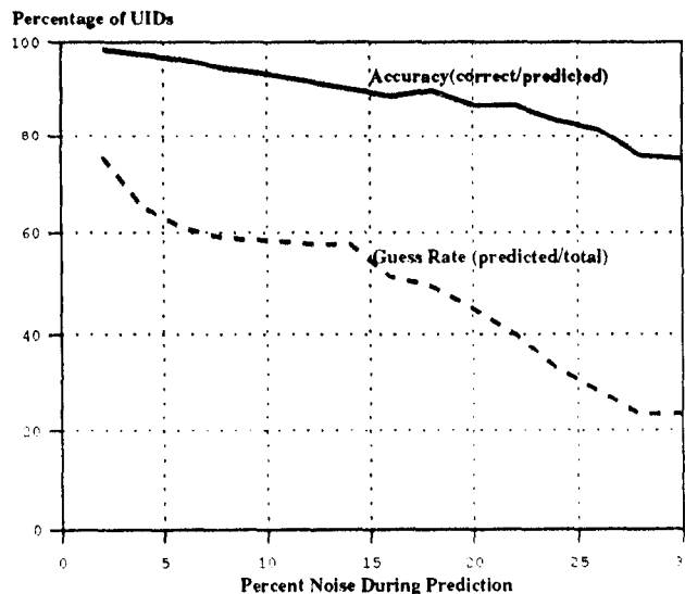
Figure 5: Prediction Accuracy and Guess Rate vs. Noise
