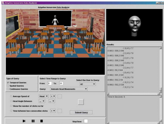
Figure 1: The main interface window of AIDA
