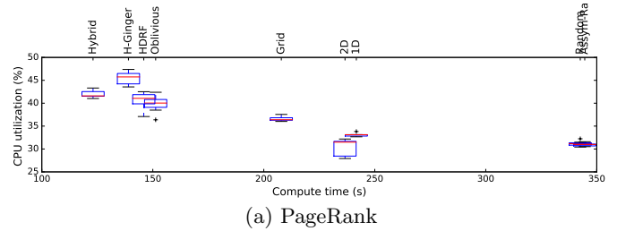
(a) PageRank
