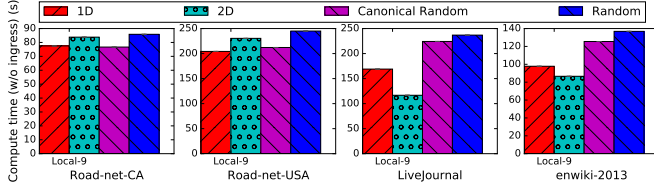
Figure 16: Computation times for PageRank on GraphX.
