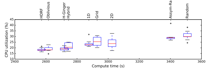
(b) K-core
