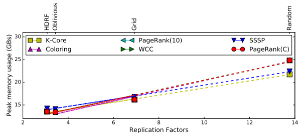
Figure 5: Memory usage vs. Replication Factors. (PowerGraph, EC2-25, UK-Web).
