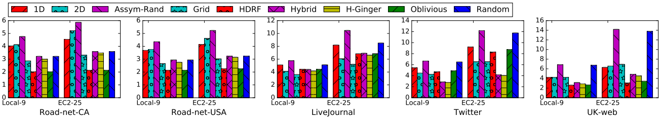
Figure 17: Replication Factors for PowerLyra with all Strategies.
