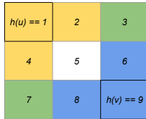
Figure 2: Grid Partitioning example: u hashes to 1, v hashes to 9. The edge (u, v) can be placed on machines 7 or 3.
