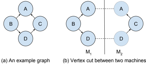
Figure 1: PowerGraph’s vertex replication model.
