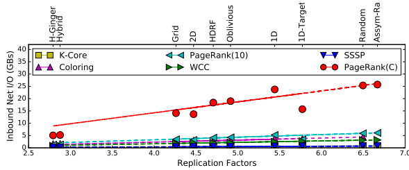
Figure 19: Incoming network IO vs. Replication Factor. (Local-9, PowerLyra, Twitter).
