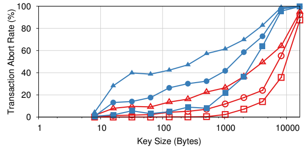
(a) Abort rate versus key size with fixed-size 8-byte payloads.
