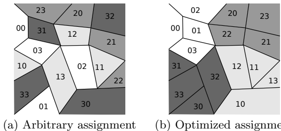
Figure 11: Centroid indexes assignment
