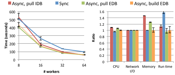
Figure 12: GalaxyEvolution: query run times and resource consumption, different cluster sizes and execution models with 32 workers. (Async, build EDB) serves as reference.
