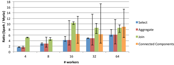
Figure 8: A comparison of Spark and MyriaX on four queries: Select ( R(x, y) :- \text{Twitter}(x, y), x < 5000000 ), aggregate ( R(x, \text{sum}(y)) :- \text{Twitter}(x, y) ), join ( R(x, z) :- \text{Twitter}(x, y), \text{Twitter}(y, z) ), and connected components . MyriaX completes these queries 1.5 \times to 10 \times faster on average than Spark. For connected components, Spark (using GraphX) runs out of memory for small cluster sizes and large data.
