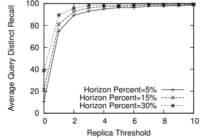
Figure 12: Average Query Distinct Recall vs Replica Threshold
