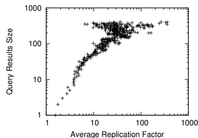
Figure 4: Correlating Query Results Size vs. Average Replication Factor.
