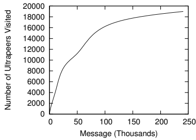
Figure 8: Gnutella Flooding Overhead
