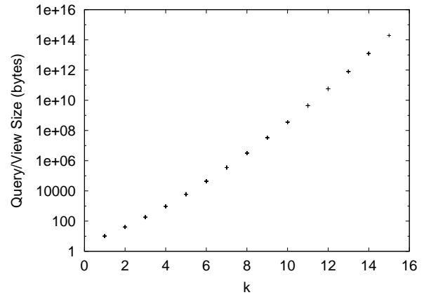
Figure 3: Growth of Q_1 and Q_2 with the multiset cardinality k .
