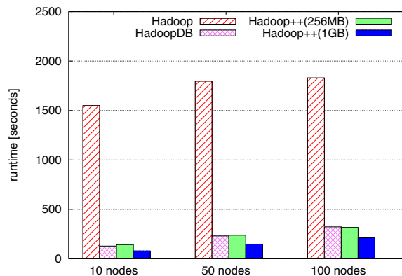
Figure 5: Runtime Improvements related to Indexing and Join Processing
