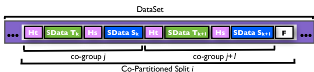
Figure 4: Co-partitioned Data Layout
