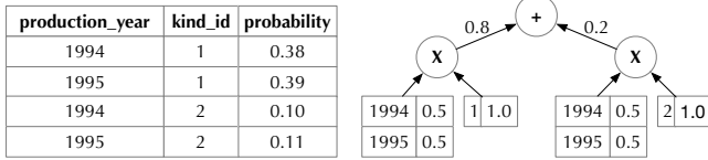
Figure 5: An example of Sum Product Network.
