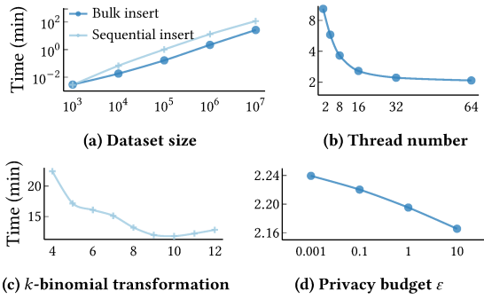
Figure 7: Inserting records under different settings. Records are inserted all at once in bulk mode and bucket by bucket in sequential mode.
