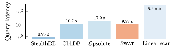
Figure 5: Range-query systems under the default setting. The security strength increases from left to right.
