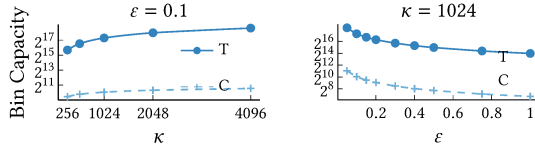
Figure 8: Minimal bin capacity obtained through the theoretical analysis (T) [14] vs. convolutional computation (C) with different security parameters \kappa and privacy budgets \epsilon .
