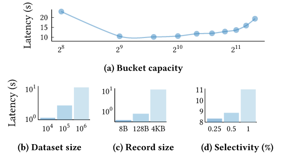
Figure 6: Query latency under different settings.
