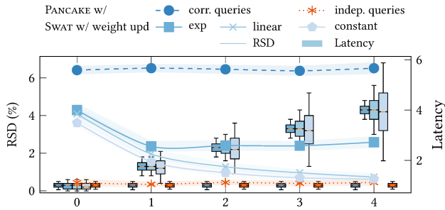
Figure 4: Privacy benefits and efficiency penalties over varying sampling pool sizes \theta and weight update policies against PANCAKE. RSD lines denotes relative standard deviation that measures the degree of dispersion of frequencies relative to the uniform. Latency bars, measured by the number of batches to retrieve the target data, serves as a key performance indicator to reflect system responsiveness. The three middle bars from left to right represent exponential, linear, and constant updates to sampling weights in each batch.
