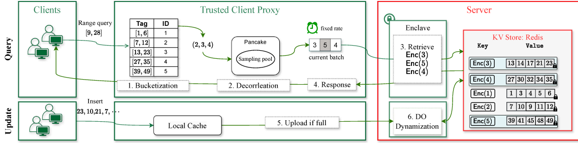
Figure 1: Upon receiving a query, the client proxy splits it into bucket accesses based on tags prepared by the cloud server’s enclave. These accesses are added to a sampling pool, from which a batch of bucket IDs is randomly selected. The proxy also filters false positives in those buckets and returns the final results to the client. Upon receiving an update, the client proxy caches it until a bucket of updates accumulates. Subsequently, the client proxy sorts these updates and uploads them to the server’s enclave. The enclave then updates the encrypted data store in a differentially oblivious way.
