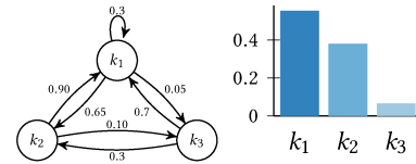
Figure 2: Markov model (left) and its stationary distribution of queried keywords (right).
