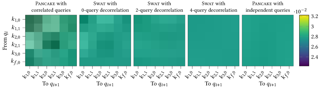
Figure 3: Observed query transition frequencies following the Markov process in Fig. 2. Reduced color variation signifies a decrease in observed query correlation. The rightmost figure represents a scenario in which queries are generated independently.
