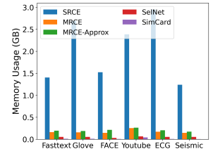
Figure 9: Memory Usage of Each Method
