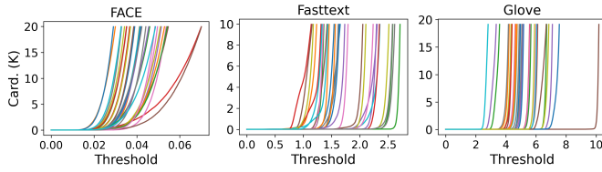
Figure 7: Cardinality Distribution of 30 Series on FACE, Fasttext, and Glove.
