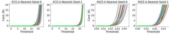
Figure 6: Cardinality Distribution of k -NN on FACE and ECG. The query series is shown in a bold, bright green line.
