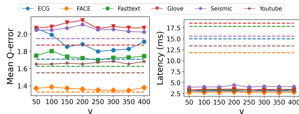
Figure 13: Parameter Study – v . The dashed line indicates the mean Q-error and selection latency of the corresponding dataset with the same color by checking the reference object candidates one by one.
