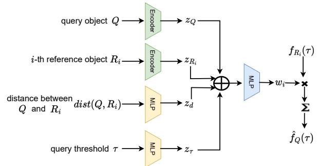
Figure 4: The Weight Estimation Model
