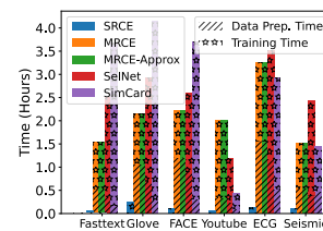
Figure 8: Offline Processing Time
