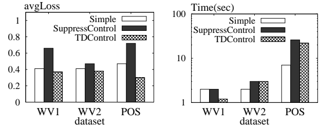
Figure 5: Varying datasets
